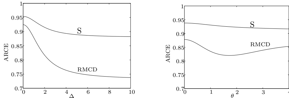
Figure 4.3. The asymptotic relative classification efficiency of Fisher's discriminant rule based on RMCD and S w.r.t. the classical method, for p = 2 , as a function of \Delta (left figure, for \theta = 0 ) and as a function of \theta (right figure, for \Delta = 1 ).
