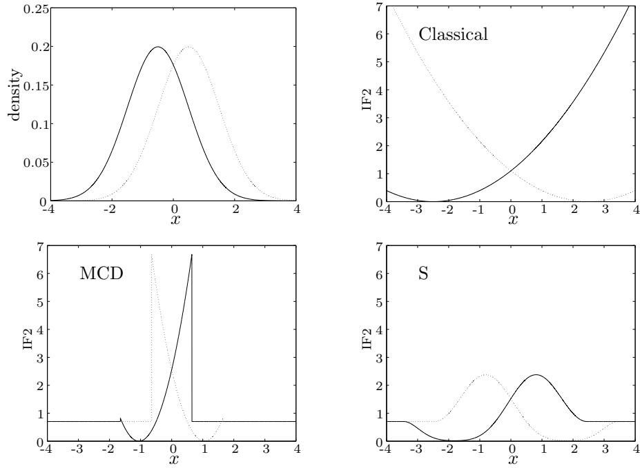
Figure 3.2. Second-order influence function of the error rate at the canonical model H_m with \pi_1 = \pi_2 , \Delta = 1 , and p = 1 , using the classical estimators (top right), the MCD (bottom left), and S-estimator (bottom right). The solid curve gives IF2 for an observation with y = 1 , the dotted line for y = 2 . The top left figures show the densities of X|Y = 1 and X|Y = 2 .
