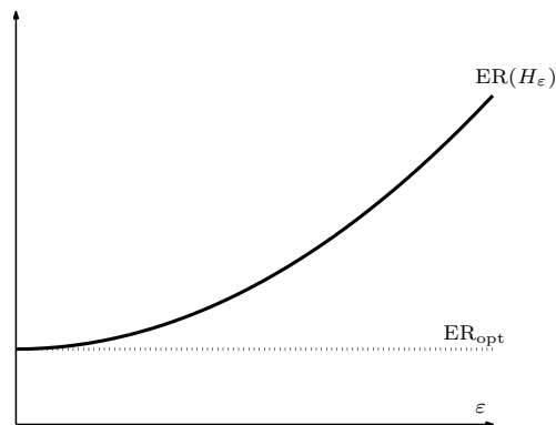
Figure 3.1. Error rate of an optimal discriminant rule based on a contaminated model distribution H_\varepsilon as a function of the amount of contamination \varepsilon .
