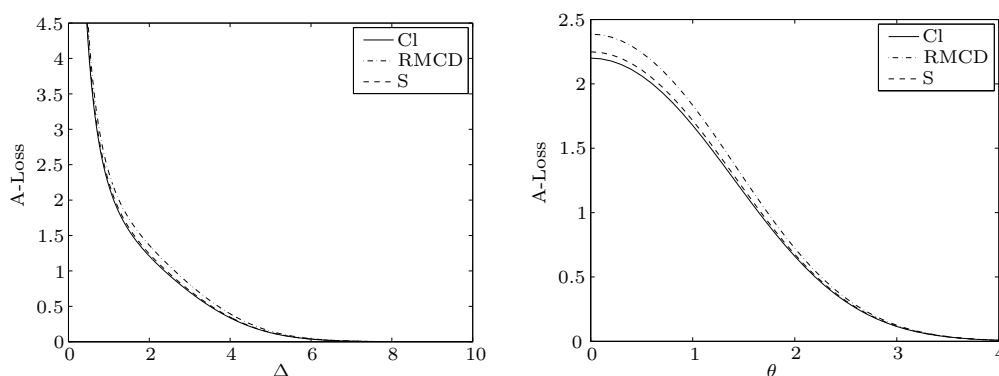
Figure 4.4. The asymptotic loss of Fisher's discriminant analysis based on the classical (solid line), on S (dashed line), and on RMCD (dashed-dotted line) estimators, for p = 5 , as a function of \Delta (left figure, for \theta = 0 ) and as a function of \theta (right figure, for \Delta = 1 ).
