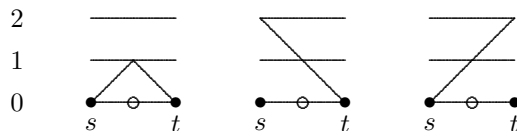
Figure 3. The three essentially different templates for r = 2 and s, t even.
