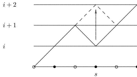
Figure 1. An admissible move at site s .
