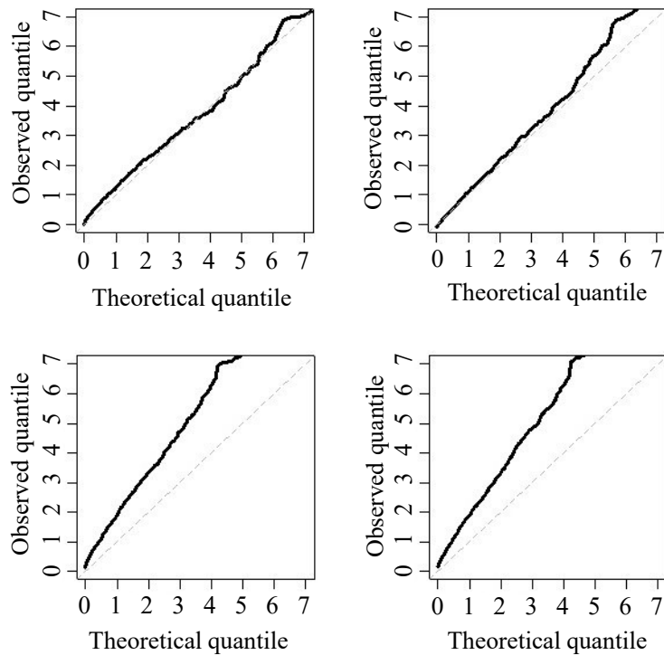
Figure 2. Quantile–quantile plots for the chi-squared distribution with one degree of freedom versus the test statistic based on Q\{\beta(s)\} (top) and Q_K\{\beta(s)\} (bottom), when the null hypothesis is true under the AR(1) (left) and compound symmetry (right) structures.
