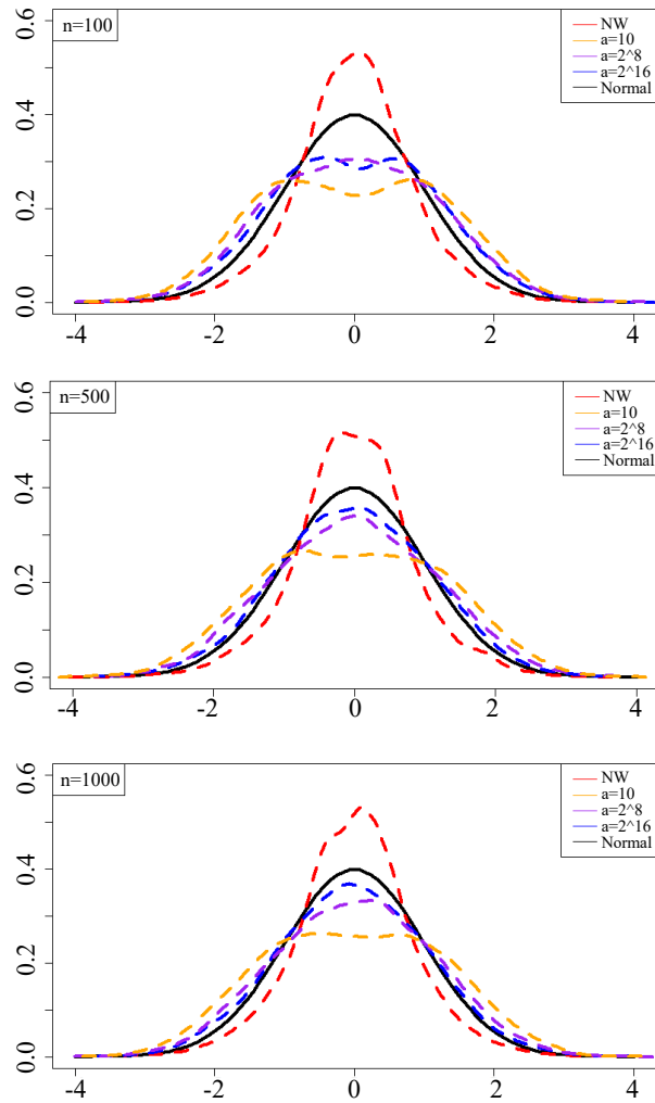
Figure 2. T_n densities under W2 with different a .
