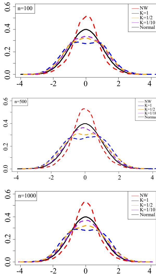
Figure 1. T_n densities under W1 with different K .
