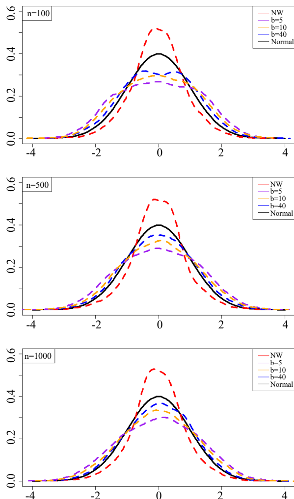
Figure 3. T_n densities under W3 with different b .
