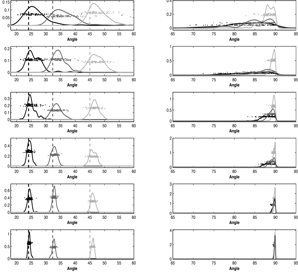
Figure A: Additional simulation plots for Example 5.1 in the main paper. Panels from top to bottom correspond to n = 50, 100, 200, 500, 1000, and 2000, respectively. In particular, the panels in the third row correspond to Figure 3 in the main paper.
