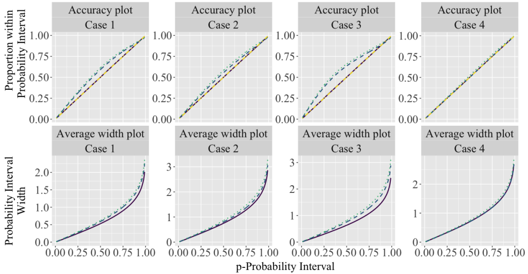
Figure 6. The accuracy plot and the average width plot computed over the validation set for interpolation ( \mathcal{V}_i ) and averaged over the 100 simulation runs.
