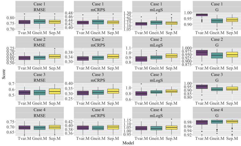
Figure 5. Boxplots of 100 simulation run-based RMSE, mCRPS, mLogS and G , computed over the forecasting validation set ( \mathcal{V}_f ).
