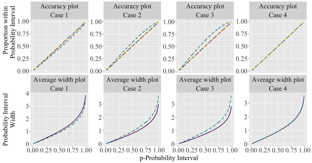
Figure 7. The accuracy plot and the average width plot computed over the validation set for forecasting ( \mathcal{V}_f ), and averaged over the 100 simulation runs.
