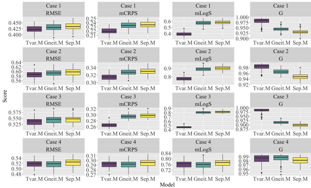
Figure 4. Boxplots of 100 simulation run-based RMSE, mCRPS, mLogS and G , computed over the interpolation validation set ( \mathcal{V}_i ).
