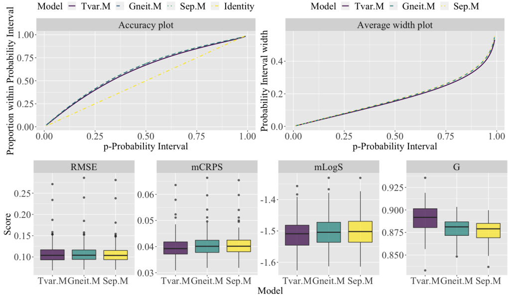
Figure 9. Prediction quality assessment metrics based on the 100 validation sets for the three candidate models. The top row shows the accuracy plot and the average width plot. The bottom row shows the boxplots of RMSE, mCRPS, mLogS and G based on the 100 runs.
