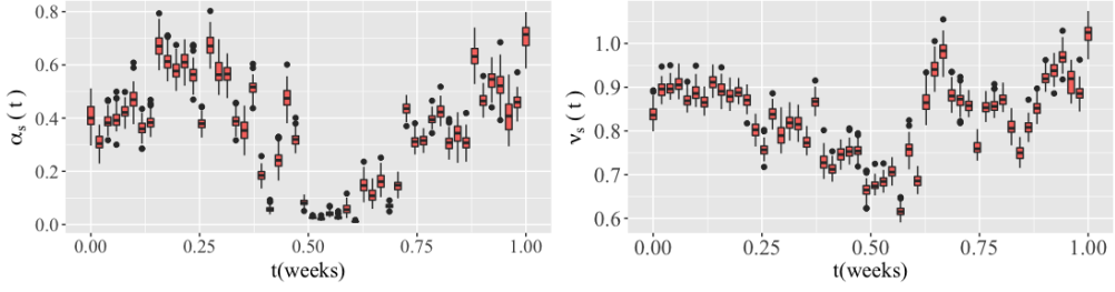
Figure 2. Boxplots illustrating the Maximum Likelihood estimates for (left) the spatial scale parameter \alpha and (right) the smoothness parameter \nu of the covariance function \sigma^2 M(\mathbf{h} \mid \alpha, \nu) . The estimates are obtained by fitting the covariance function independently over the standardized residuals for each week on the 100 training sets.
