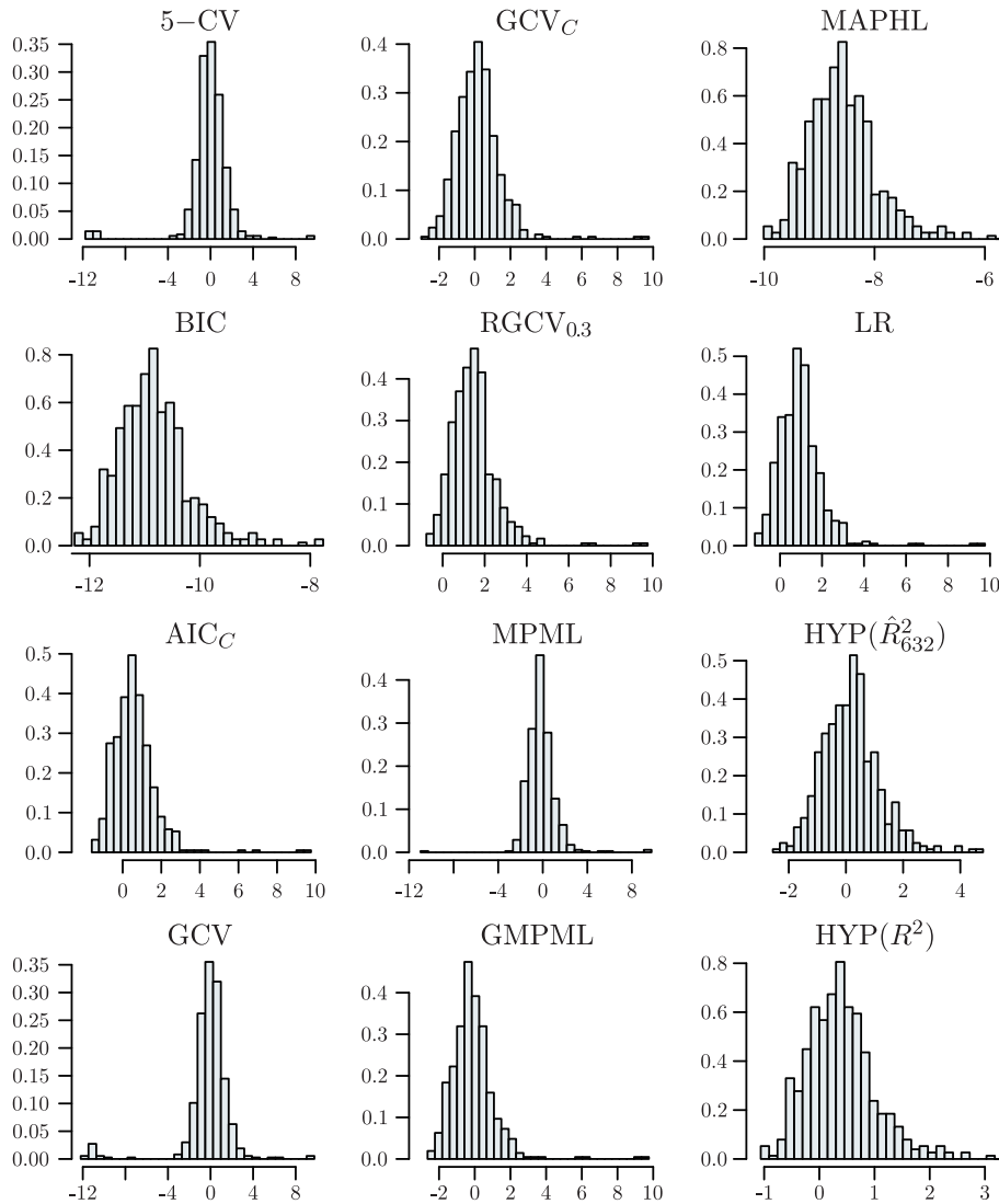
Figure 3. Histograms of \ln(\lambda/\lambda_{\text{opt}}) for p=4,000 , n=100 , \pi=0.3 , R^2=0.2 , and correlated covariates. \ln(\lambda/\lambda_{\text{opt}}) = 0 means that \lambda was chosen to yield optimal shrinkage. All methods are described in Table 1.
