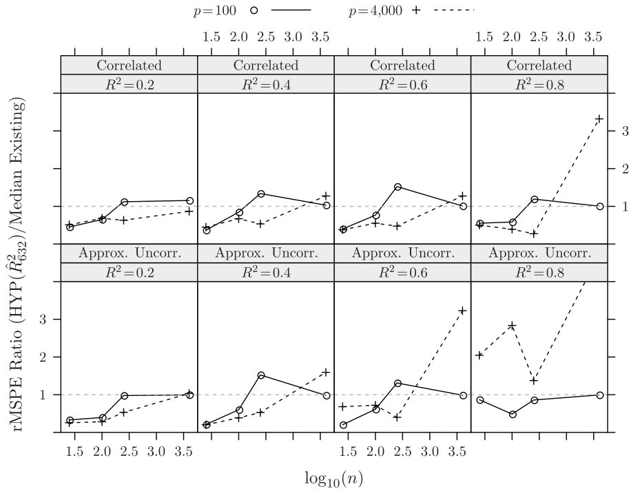
Figure 1. Ratio of the rMSPE of HYP( \hat{R}_{632}^2 ) to the median rMSPE of remaining methods, excluding GCV C , over \log_{10}(n) . Values less than one indicate that HYP( \hat{R}_{632}^2 ) has smaller prediction error.
