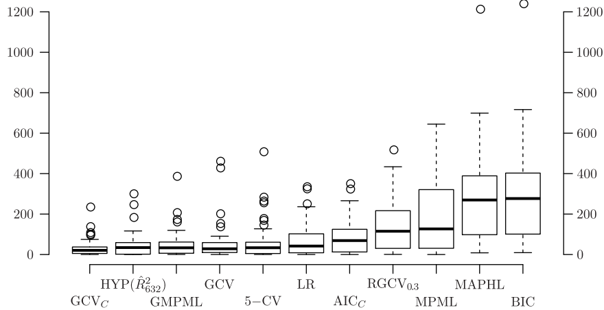
Figure 4. Boxplots of rMSPEs from 1,000 training/testing partitions of the Bardet-Biedl data, ordered from left to right in terms of average rMSPE.
