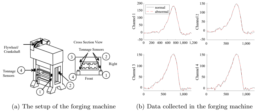
Figure 1. Forging machine setup and the collected tonnage data set.
