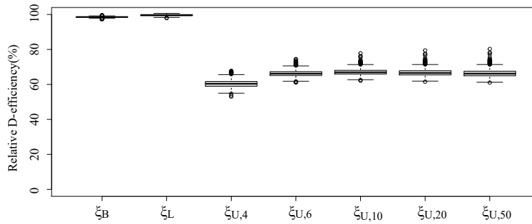
Figure 1. Summary of the relative D -efficiencies of the Bayesian optimal design ( \xi_B ), locally optimal design ( \xi_L ), and the uniform-weights designs ( \xi_{U,k} ).
