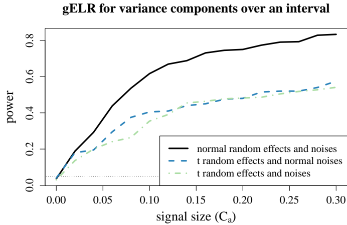
Figure 3. Empirical power for the global test H_0 : \sigma_A^2(t) \equiv 0, t \in [0, 1] at different values of C_a . The dotted horizontal line is the nominal threshold 0.05.
