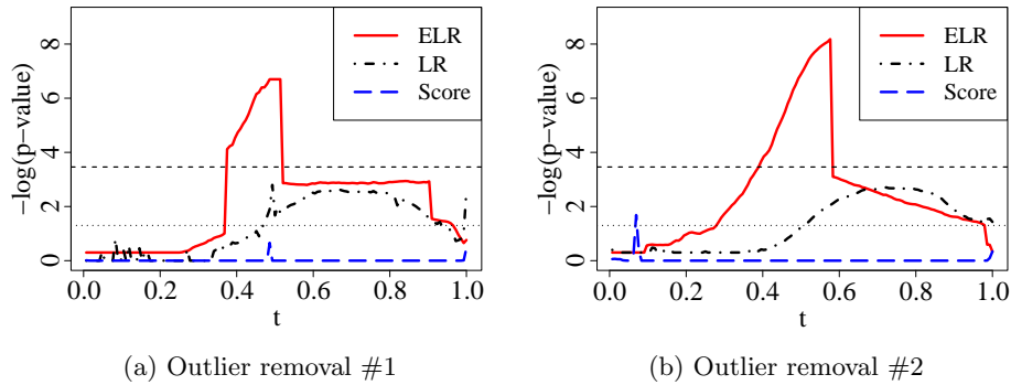
Figure 6. The -\log_{10}(p\text{-value}) of testing heritability H_0 : \sigma_A^2(t) = 0 for different quantile values t . The dotted horizontal line is the nominal threshold -\log_{10}(0.05) , and the dashed horizontal line is the Bonferroni corrected threshold -\log_{10}(0.05/144) .
