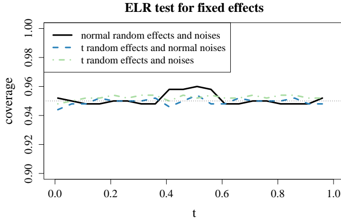
Figure 1. Coverage probability for the ELR test for fixed effects. The dotted horizontal line is the 95% coverage probability.
