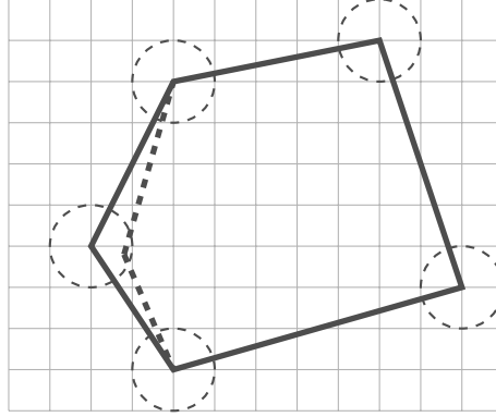
Figure S2: Effect of perturbation of vertices of a polygon.
