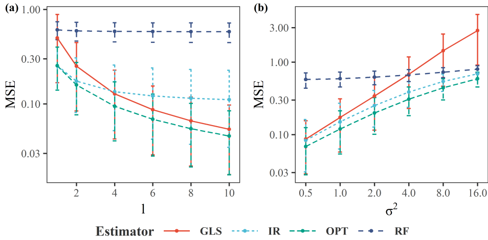
Figure 4. Empirical means and the 10th, 90th quantiles of the MSEs (in the log-scale), in the presence of the random effects, calculated from 1,000 simulation replications for the GLS, the inverse regression (IR), the optimal shrinkage (OPT) and the inverse regression with the random forest (RF) estimators with respect to the numbers of repeated measurements l (a) and different scales of noises \sigma^2 .
