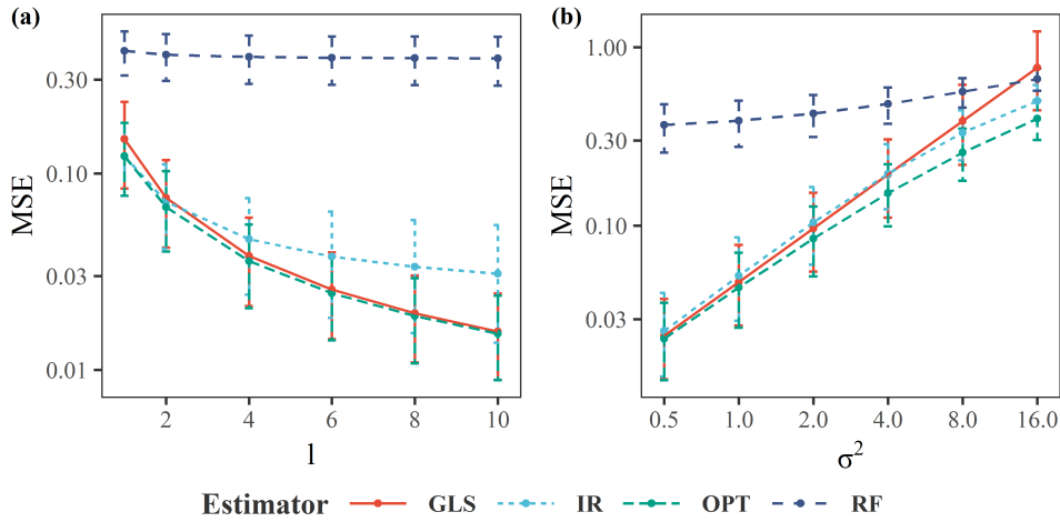
Figure 2. Empirical means and the 10th, 90th quantiles of the MSEs (in log-scale) calculated from 1,000 simulation replications for the GLS, the inverse regression (IR), the optimal shrinkage (OPT) and the inverse regression with the random forest (RF) estimators with respect to numbers of repeated measurements l (a) and the variances of the noises \sigma^2 (b).
