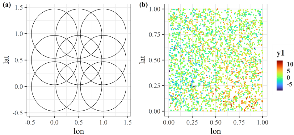
Figure 3. (a) Nine “bisquare” basis functions whose center points are evenly located in the square region [0, 1] \times [0, 1] . (b) Locations of the 2500 individuals, where the colors indicate the value of the first dependent variable y_1 . It is clear that y_1 has a correlation structure among the individuals.
