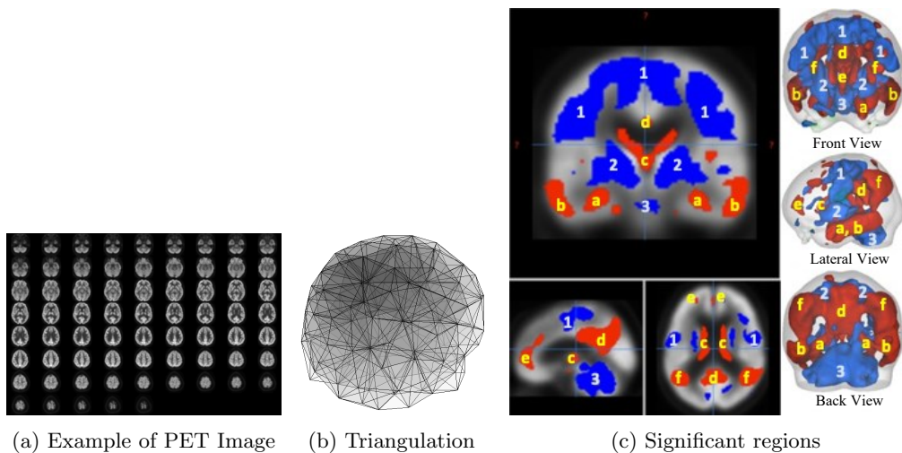
Figure 4. (a) An example of a PET image; (b) the triangulated domain of a human brain; and (c) visual representation of significant regions in the comparison between subjects in the CON and AD groups, based on the coverage of zero by the SCC. The regions marked in red indicate areas where zero exceeds the upper SCC threshold, while regions in blue indicate areas where zero falls below the lower SCC threshold.
