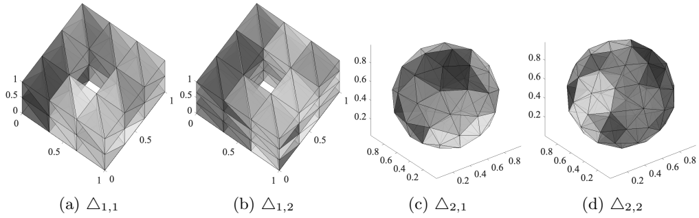
Figure 1. Triangulation of domain \Omega_1 and \Omega_2 .
