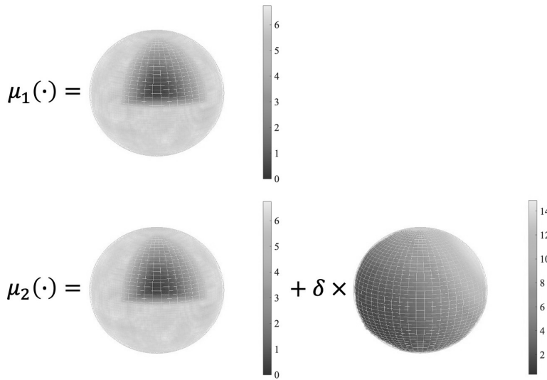
Figure 2. Design of \mu_1 and \mu_2 in the simulation study of two-sample SCC.
