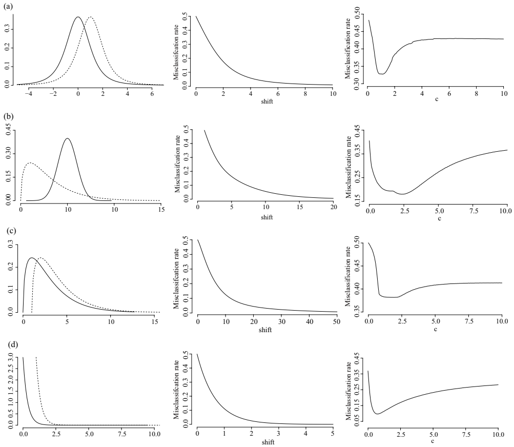
Figure 2. Misclassification rates in four different settings. The probability density functions of two populations are shown in each panel of the first column; each panel of the second column depicts the misclassification rate as the function of d assuming \sigma_1 = \sigma_2 ; The misclassification rate as a function of c = \sigma_2/\sigma_1 is shown in the last column. (a) location-shifted Gaussians; (b) a Gaussian distribution and a chi-squared distribution; (c) location-shifted chi-squared distributions; (d) location-shifted exponentials.
