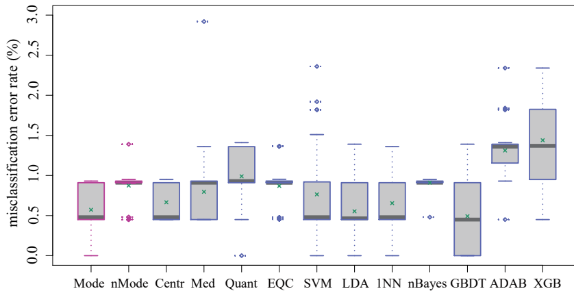
Figure 4. Box plots of misclassification error rates for DNA methylation dataset.
