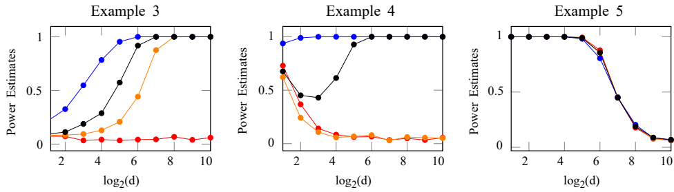
Figure 2. Powers of \text{BD-}\ell_2(\bullet) , \text{BD-}\ell_1(\bullet) , \text{BD-exp}(\bullet) and \text{BD-log}(\bullet) in Examples 3–5.
