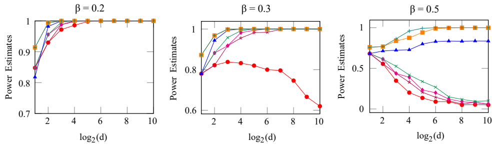
Figure 3. Powers of the \text{BD-}\ell_2 test for different choice of \beta (0.2, 0.3 and 0.5) and \gamma (0 (●), 0.4 (★), 0.5 (◆), 0.6 (×), 0.9 (▲), 1 (■), 1.1 (+)).
