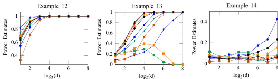
Figure 8. Powers of \text{BD-}\ell_2 (●), \text{BD-}\ell_1 (○), \text{BD-exp} (●), \text{BD-log} (●), \text{FR} (■), \text{BF} (◆), \text{NN} (■), \text{MMD} (◆), \text{SHP} (■), \text{BG} (◆) tests in Examples 12–14.
