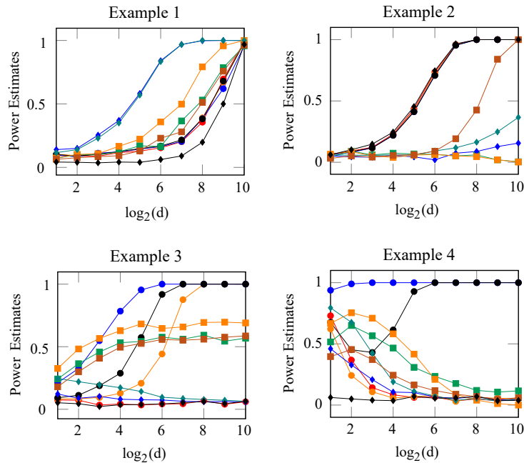
Figure 5. Powers of \text{BD-}\ell_2 (●), \text{BD-}\ell_1 (○), \text{BD-exp} (●), \text{BD-log} (●), \text{FR} (■), \text{BF} (◆), \text{NN} (■), \text{MMD} (◆), \text{SHP} (■), \text{BG} (◆) tests in Examples 1–4.
