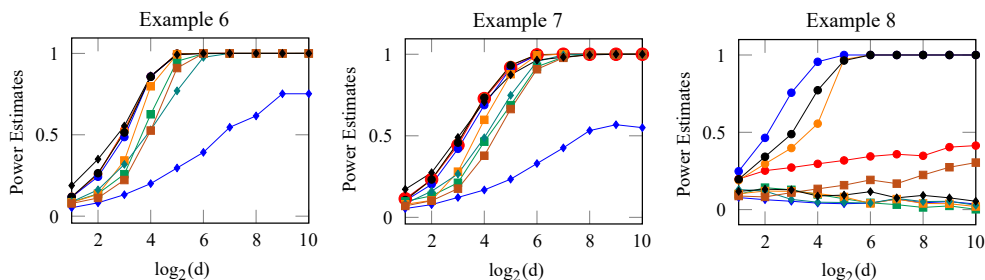
Figure 6. Powers of \text{BD-}\ell_2 (●), \text{BD-}\ell_1 (○), \text{BD-exp} (●), \text{BD-log} (●), \text{FR} (■), \text{BF} (◆), \text{NN} (■), \text{MMD} (◆), \text{SHP} (■), \text{BG} (◆) tests in Examples 6–8.
