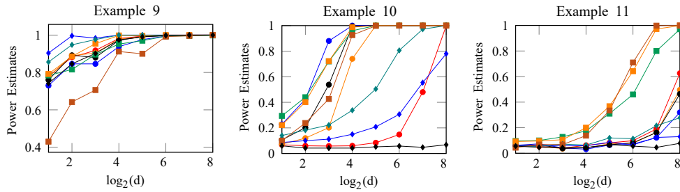
Figure 7. Powers of \text{BD-}\ell_2 (●), \text{BD-}\ell_1 (○), \text{BD-exp} (●), \text{BD-log} (●), \text{FR} (■), \text{BF} (◆), \text{NN} (■), \text{MMD} (◆), \text{SHP} (■), \text{BG} (◆) tests in Examples 9–11.
