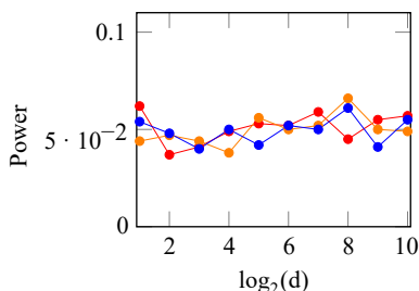
Figure 4. Observed levels of BD- \ell_2 test for n = m = 20 (●), 35 (●) and 50 (●).
