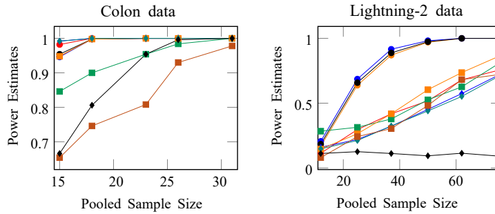
Figure 9. Powers of \text{BD-}\ell_2 (●), \text{BD-}\ell_1 (○), \text{BD-exp} (●), \text{BD-log} (●), \text{FR} (■), \text{BF} (◆), \text{NN} (■), \text{MMD} (◆), \text{SHP} (■), \text{BG} (◆) tests in benchmark data sets.
