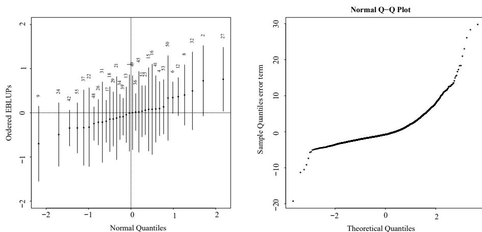
Figure 1. Normal QQ-plots for the EBLUPs \hat{\alpha}_i and estimated errors \hat{e}_{ij} from the model (5.1) fitted to the consumer expenditure on fresh milk products in 2002 data.
