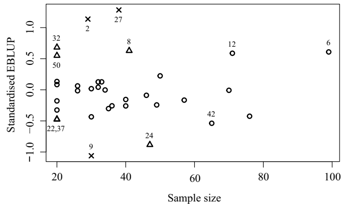
Figure 2. Plot of the population standardised EBLUPS \hat{\alpha}_i/\hat{\sigma}_\alpha against sample size in each state for the consumer expenditure on fresh milk products. Group 1 states are plotted as circles, Group 2 as triangles and Group 3 as crosses. Selected states are labelled by state number.
