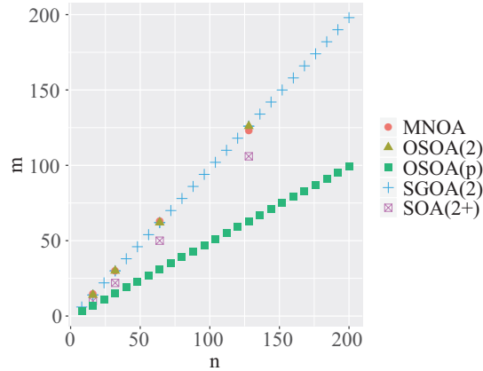
Figure 1. Comparison of SGOAs of strength 2 with some related designs for s = 2 .
