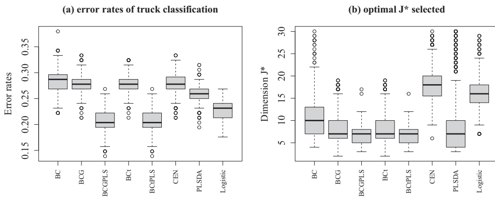
Figure 5. Box plots of misclassification rates and optimal number of components J^* in the truck emission case over 1,000 repetitions of 10-fold cross-validation. BCt-PLS and BCG-PLS achieve the lowest average error rate with J^* concentrated around 7.
