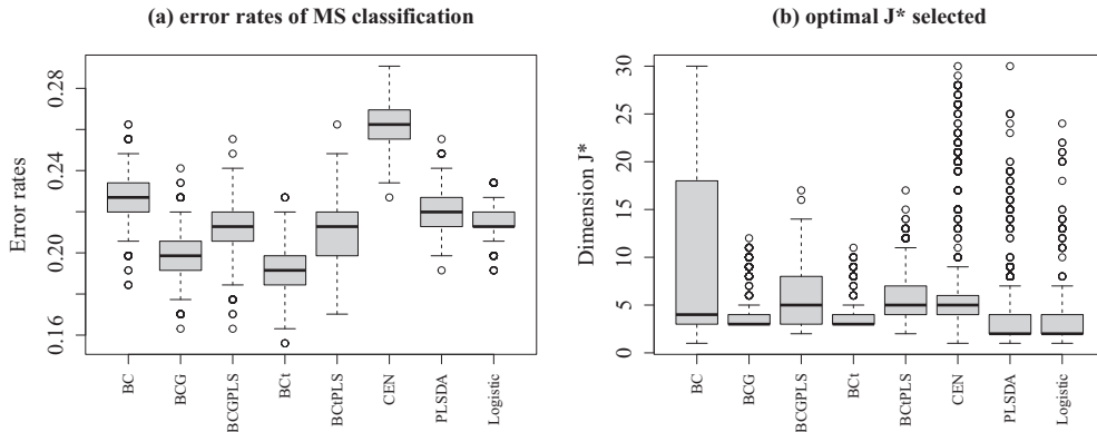
Figure 3. Box plots of misclassification rates and optimal number of components J^* in the MS study over 1,000 repetitions of 10-fold cross-validation. BCt achieves the lowest average error rate, while requiring a very small number of components ( J^* < 5 ) with lowest variation.
