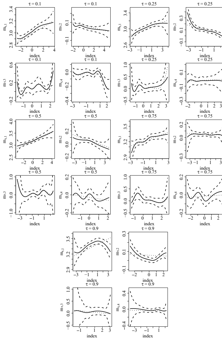
Figure 2. Plots of the unpenalized estimator \hat{m}_l(\cdot) (solid line) and its 95% pointwise confidence intervals (dashed line), and the penalized estimator \tilde{m}_l(\cdot) (dotted line).
