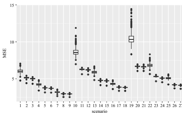
Figure 3. Empirical MSE in predicting X for FECA designs (*) vs. 1,000 random designs (box plot) with \sigma^2 = 10 .
