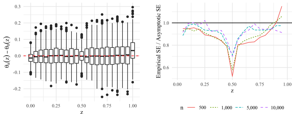
Figure 1. Left: Box plots of \theta_n^*(z) - \theta_0(z) with n = 10K . Right: Empirical standard errors of r_n[\theta_n^*(z) - \theta_0(z)] divided by the limit theory-based counterparts for z \in (0, 1) , where r_n = n^{1/2} for z = 0.5 , and r_n = n^{1/3} otherwise.
