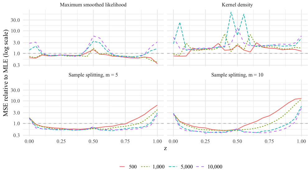
Figure 2. Relative mean squared errors of the maximum smoothed likelihood estimator, kernel density-based estimator, and sample splitting estimators to the maximum likelihood estimator for z \in [0, 1] and various sample sizes n . The maximum likelihood has a better mean squared error for y -values greater than one, and the other estimator has a better mean squared error for y -values less than one.
