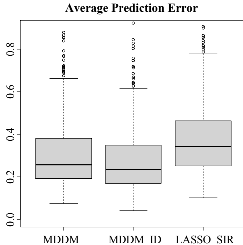
Figure 2. The averaged prediction error over 500 training-testing sample splits and over q = 15 response variables.
