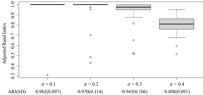
Figure 2. Average adjusted rand index between the clustering results using the estimated \hat{\Theta}Z and using the true \Theta_0 Z , respectively, for different values of \sigma .
