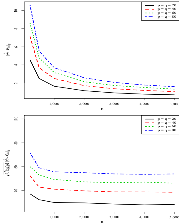
Figure 1. Estimation error \|\text{vec}(\hat{\Theta} - \Theta_0)\|_2 for different values of p = q as n increases.
