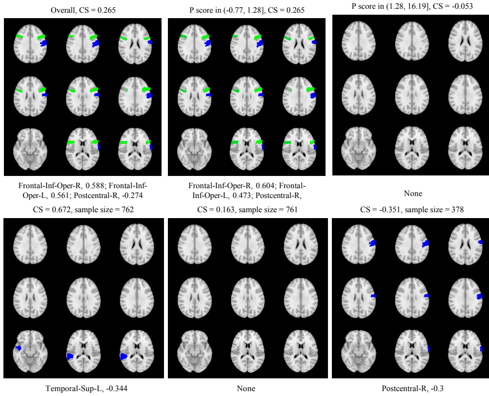
Figure 5. Association patterns between brain regions and cognitive outcome for different subgroups. The top row is for the entire study cohort, the group with the psychological score lower than the threshold, and the group higher than the threshold. The bottom row is for the three subgroups identified by K -means applied to \Theta \mathbf{Z}_i . Significant positive and negative associations are represented by green and blue colors, respectively, for corresponding brain regions.
