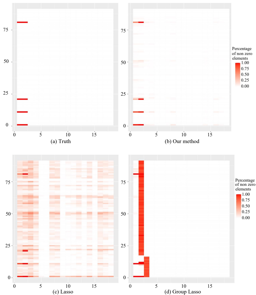
Figure 3. (a) Heat map of the true nonzero entries, (b) the estimated nonzero entries by our method, (c) the entry-wise Lasso , and (d) column-wise group Lasso.
