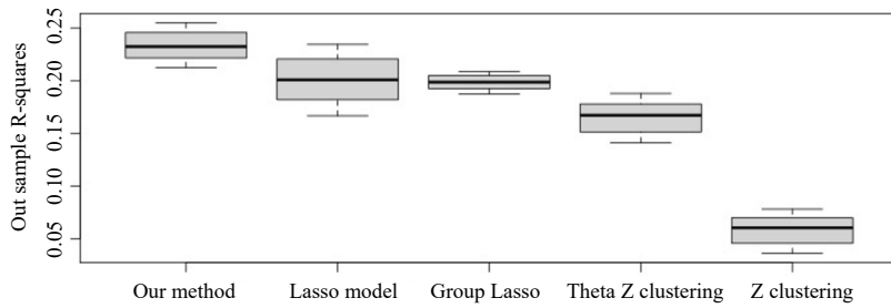
Figure 6. Prediction performance in terms of R^2 from 100 random data splits. The mean and the standard deviation are shown in the bottom row.
