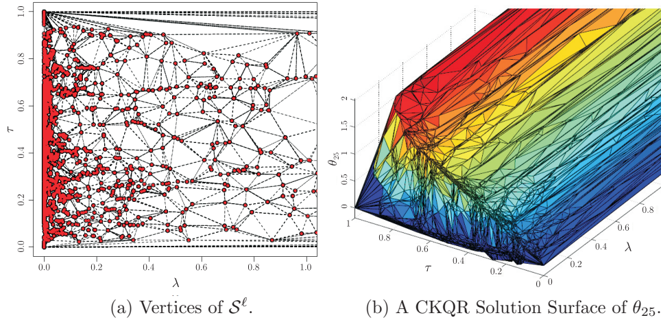
Figure 1. Two-dimensional solution surfaces of CKQR for the lung data: (a) shows vertices and edges of the \mathcal{S}^\ell s produced from the proposed algorithm and (b) depicts the solution surface of \hat{\theta}_{25} .
