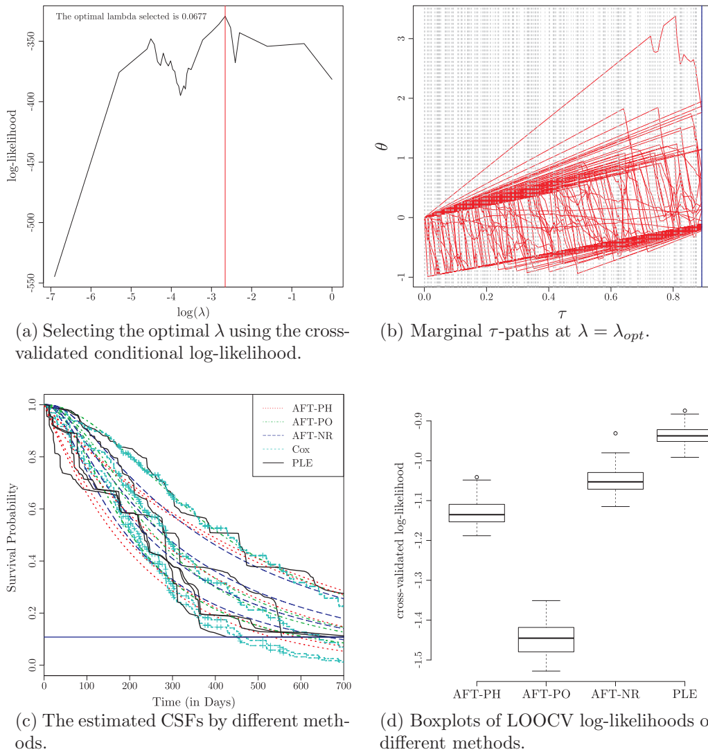
Figure 2. Conditional survival function estimator for lung Data: the panel (a) shows cross-validated conditional log-likelihood for different \lambda and the (red) vertical line represents the selected optimal \lambda_{opt} ; (b) depicts solution paths of \hat{\theta}_1, \dots, \hat{\theta}_{48} as a function \tau \in [0, \tau_0] at \lambda_{opt} where \tau_0 is estimated by 0.892 at a cutoff value of \gamma = 0.05 (blue solid vertical line); (c) shows estimated CSFs for the first five patients and the results look similar; (d) depicts boxplots of LOOCV log-likelihoods computed from different CSF estimates and PLE outperforms all others.
