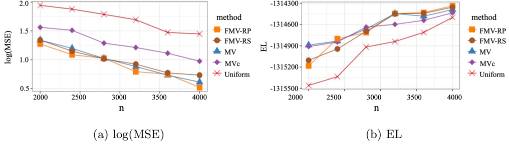
Figure 3. The log of MSE and EL based on MV, MVc, FMV-RP, FMV-RS, and Uniform methods, where n_0 = 1000 , \rho = 0.2 , r_1 = r_2 = 20000 , r_3 = 4 .
