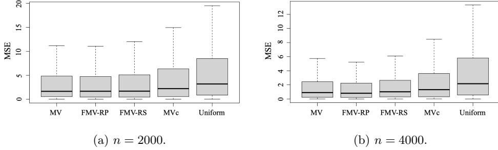
Figure 4. The MSE based on MV, MVc, FMV-RP, FMV-RS, and Uniform methods, where n_0 = 1000 , \rho = 0.2 , r_1 = r_2 = 20000 , r_3 = 4 .
