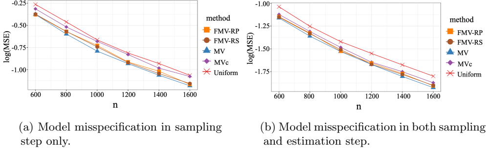
Figure 2. The log of MSE for the model misspecification scenarios with different n based on MV, FMV-RP, FMV-RS, MVc, and Uniform methods, where n_0 = 400 , \rho = 0.2 , r_1 = r_2 = 5000 , r_3 = 10 .
