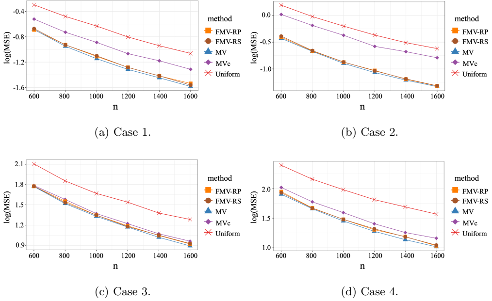
Figure 1. The log of MSE for Model (6.1) with different n based on MV, FMV-RP, FMV-RS, MVc, and Uniform methods, where n_0 = 400 , \rho = 0.2 , r_1 = r_2 = 5000 , r_3 = 10 .
