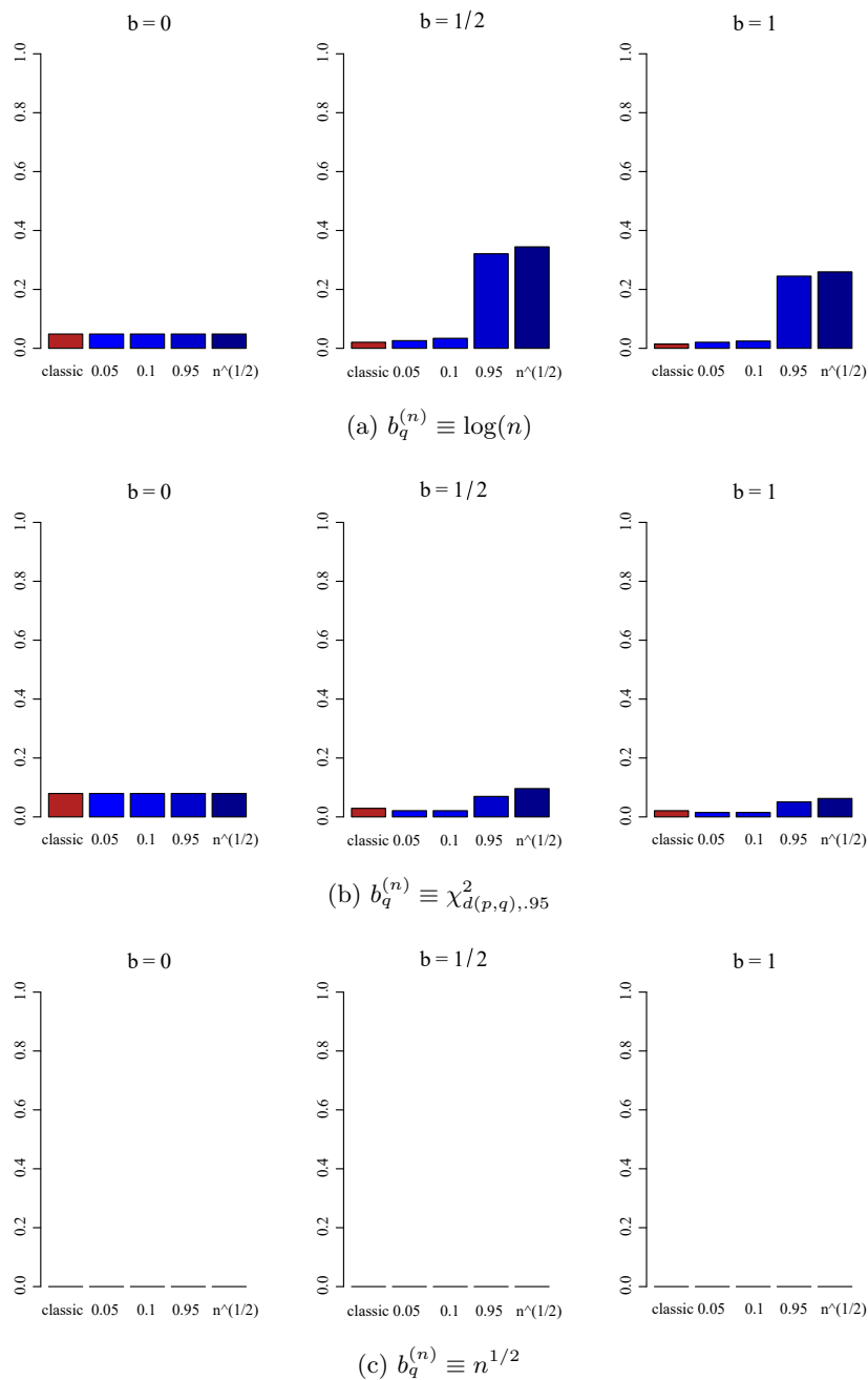
Figure 6. Proportion of good selection of k for three estimators \hat{k} (in red, denoted as “classic”) and for estimators \hat{k}_{\text{new}} (in blue) with b_q^{(n)} \in \{\log(n), \chi_{d(p,q),.95}^2, n^{1/2}\} , and c^{(n)} \in \{\chi_{2;.05}^2, \chi_{2;.1}^2, \chi_{2;.95}^2, n^{1/2}\} . The sample size is n = 1000 and \tau^{(n)} = n^{-1/2} .
