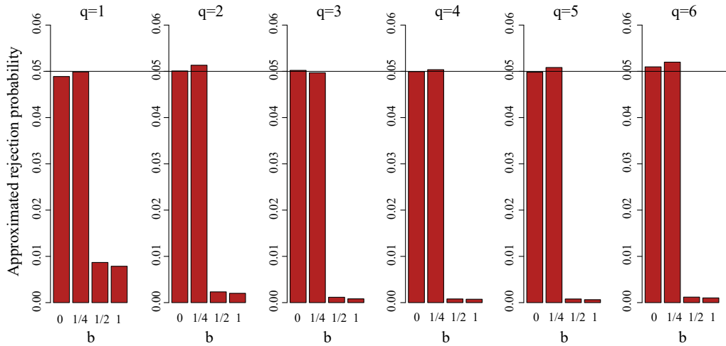
Figure 2. Approximations of \lim_{n \rightarrow \infty} E(\phi^{(n)}) for p = 8 and various values of q under triangular arrays of observations with covariance \Sigma^{(n)}(b) = \text{diag}\{(1 + n^{-b})\mathbf{1}_q, \mathbf{1}_{p-q}\} . The test \phi^{(n)} is performed at the nominal level \alpha = 0.05 . The approximation is based on 100,000 replications of the random variable in (3.3).
