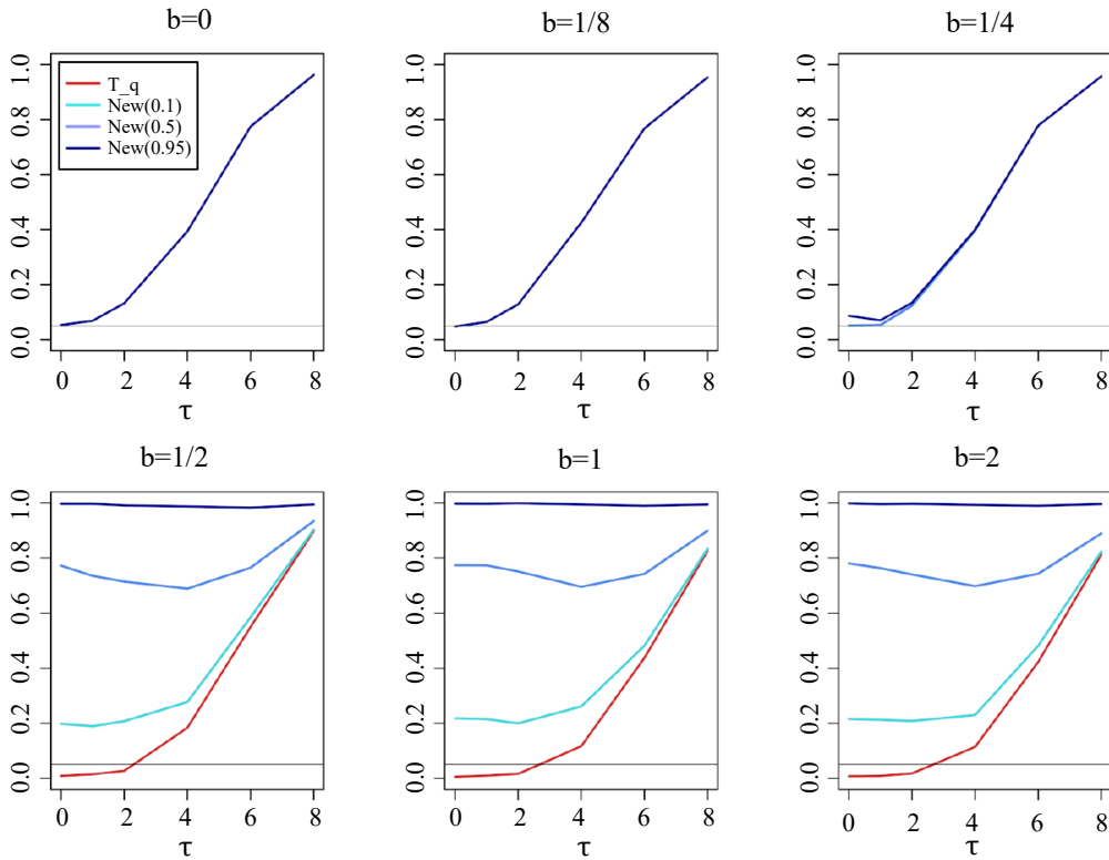
Figure 4. Empirical rejection frequencies of the classical \phi^{(n)} performed at the asymptotic nominal level 0.05 and three versions of the \phi_{\text{new}}^{(n)} test (all with \alpha = 0.05 in (5.1)), based on three different choices of \gamma : \gamma = 0.9 (denoted as new(.1)), \gamma = 0.5 (denoted as new(0.5)), and \gamma = 0.05 (denoted as new(0.95)). The sample size is n = 10,000 .
