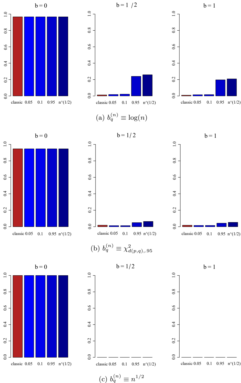
Figure 5. Proportion of good selection of k for three estimators \hat{k} (in red, denoted as “classic”) and for estimators \hat{k}_{\text{new}} (in blue) with b_q^{(n)} \in \{\log(n), \chi^2_{d(p,q),.95}, n^{1/2}\} , and c^{(n)} \in \{\chi^2_{2;.05}, \chi^2_{2;.1}, \chi^2_{2;.95}, n^{1/2}\} . The sample size is n = 1000 and \tau^{(n)} = 0 .
