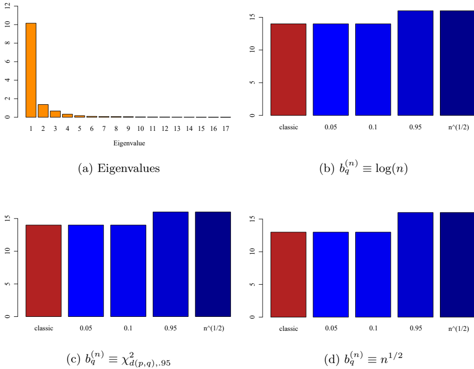
Figure 8. (a) the eigenvalues of the log-transformed gene expression data set; (b)-(d) the values (between zero and 16) taken by the estimators \hat{k} (in red, denoted as “classic”) for b_q^{(n)} \in \{\log(n), \chi^2_{d(p,q),0.95}, n^{1/2}\} and \hat{k}_{\text{new}} (in blue) for b_q^{(n)} \in \{\log(n), \chi^2_{d(p,q),0.95}, n^{1/2}\} and c^{(n)} \in \{\chi^2_{2;0.05}, \chi^2_{2;0.1}, \chi^2_{2;0.95}, n^{1/2}\} .
