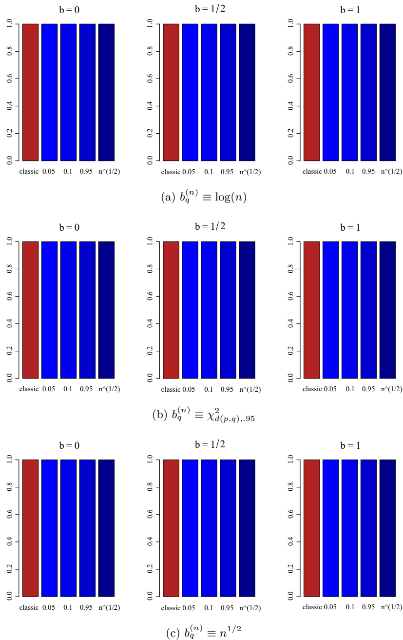
Figure 7. Proportion of good selection of k for three estimators \hat{k} (in red, denoted as “classic”) and for estimators \hat{k}_{\text{new}} (in blue) with b_q^{(n)} \in \{\log(n), \chi^2_{d(p,q),.95}, n^{1/2}\} , and c^{(n)} \in \{\chi^2_{2;0.05}, \chi^2_{2;.1}, \chi^2_{2;0.95}, n^{1/2}\} . The sample size is n = 1000 and \tau^{(n)} = 0.99 .
