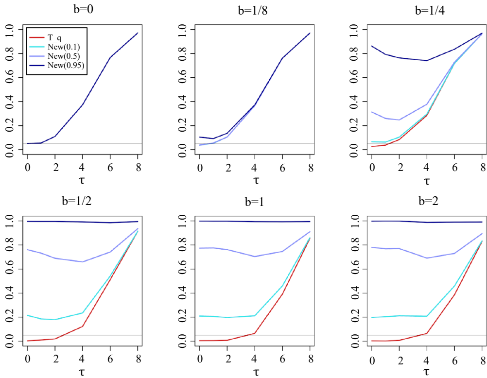
Figure 3. Empirical rejection frequencies of the classical \phi^{(n)} performed at the asymptotic nominal level 0.05 and three versions of the \phi_{\text{new}}^{(n)} test (all with \alpha = 0.05 in (5.1)), based on three choices of \gamma : \gamma = 0.9 (denoted as new(0.1)), \gamma = 0.5 (denoted as new(0.5)), and \gamma = 0.05 (denoted as new(0.95)). The sample size is n = 500 .
