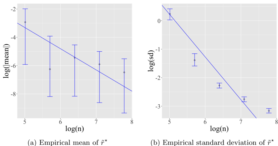
Figure 1. Plots for logistic regression illustrating order of \tilde{r}^* (5.3). The mean, and the standard deviation functions of n , are plotted against \log(n) along with bootstrap 95% confidence intervals. The solid line has slope -3/2 and the intercept is fitted using the least squares estimate.
