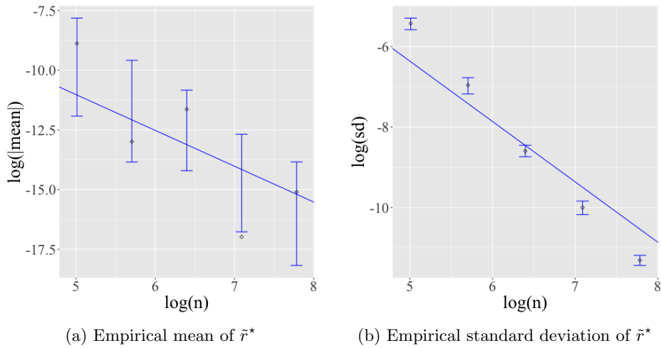
Figure 2. Plots for t_5 based regression illustrating the order of \tilde{r}^* (5.3). The mean, and the standard deviation functions of n , are plotted against \log(n) along with bootstrap 95% confidence intervals. The solid line has slope -3/2 and the intercept is fitted using the least squares estimate.
