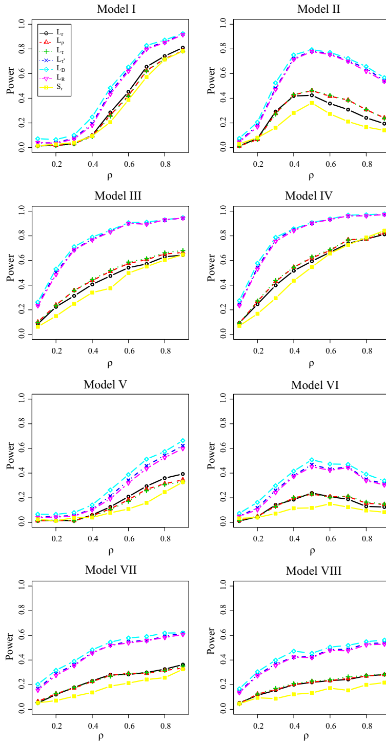
Figure 1. Power curves of different methods with different \rho and k_0 = 2, n = 100, p = 30, K = 2 .
