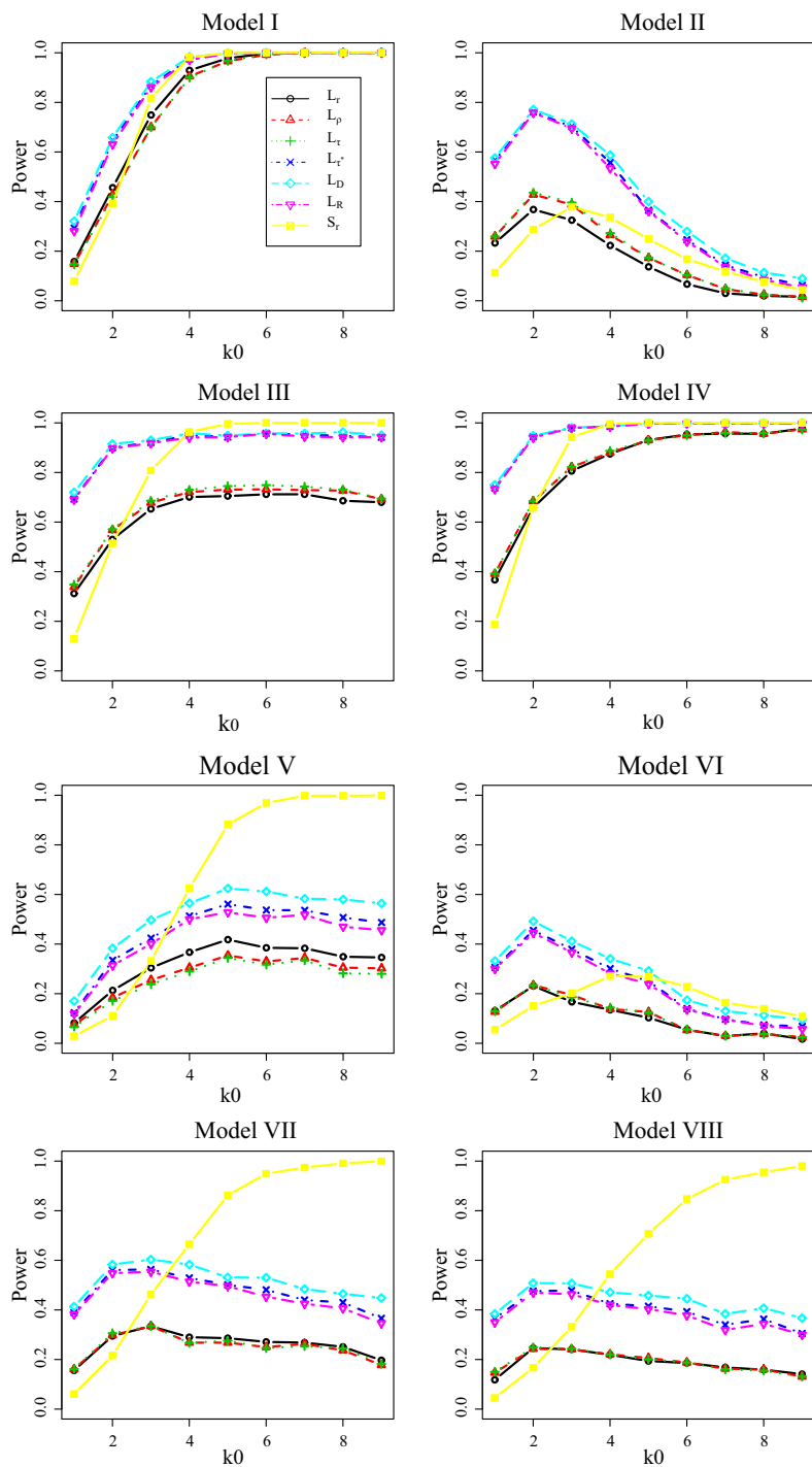
Figure 2. Power curves of different methods with different k_0 and \rho = 0.6, n = 100, p = 30, K = 2 .
