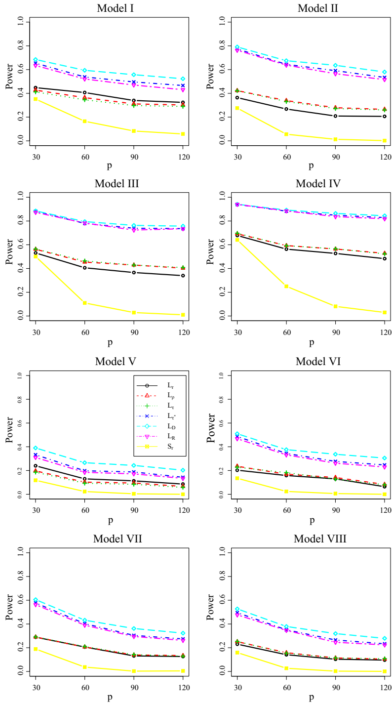
Figure 3. Power curves of different methods with different p and \rho = 0.6, n = 100, k_0 = 2, K = 2 .
