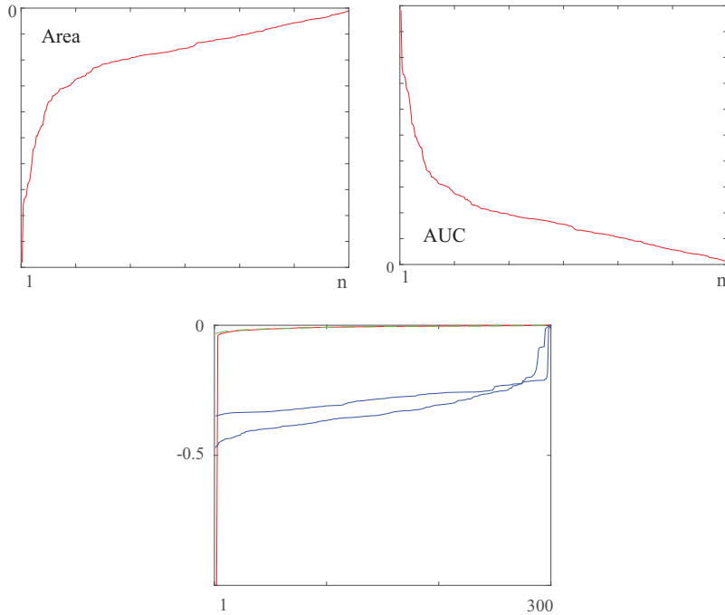
Figure 2. Left panel: example plot of s_\alpha(\mathbf{w}_i) with labeled Area; Middle panel: example plot of |s_\alpha(\mathbf{w}_i)| with AUC_\alpha labeled AUC; Right panel: simulation plot of s_\alpha(\mathbf{w}_i) for dimensions k = 1, 2, 3, 4 with d = 2 .
