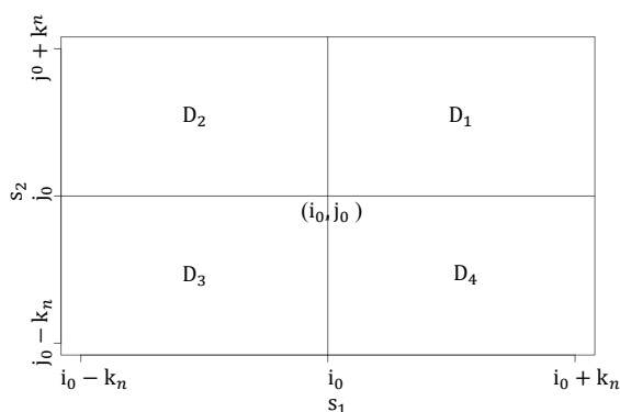
Figure 1. Blocks D_l(i_0, j_0) , l = 1, \dots, 4 , for a point (i_0, j_0) .
