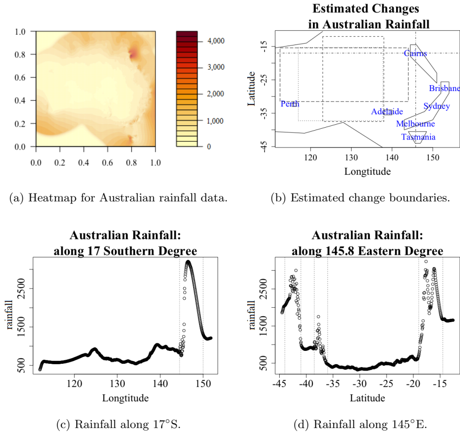
Figure 7. Heatmaps, estimated change boundaries and some 1-d examples of Australian rainfall. In the heatmap (a), the left-bottom point is ( 45^{\circ} S, 112^{\circ} E) and the right-upper point is ( 10.5^{\circ} S, 155^{\circ} E).
