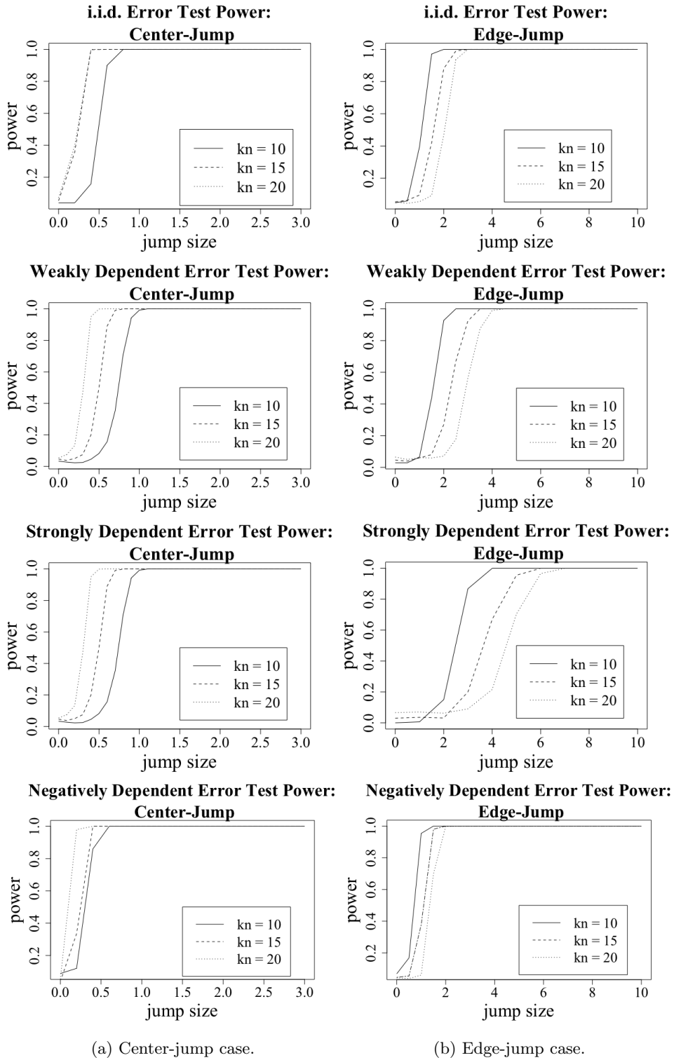
Figure 4. Test power against jump size for various k_n using the extreme-value test statistic.
