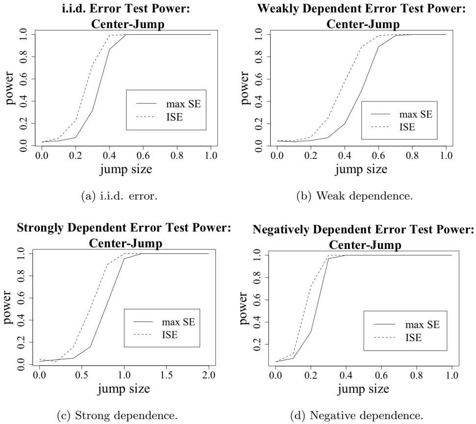
Figure 3. Tradeoff in center-jump case.
