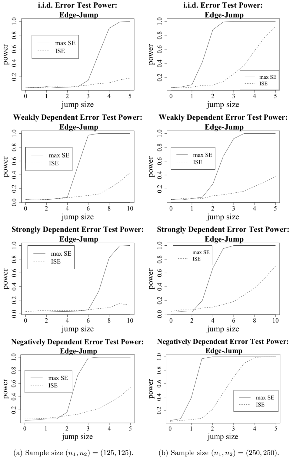
Figure 2. Test power against jump size for the i.i.d., weakly dependent, strongly dependent and negatively dependent error term, edge-jump case.
