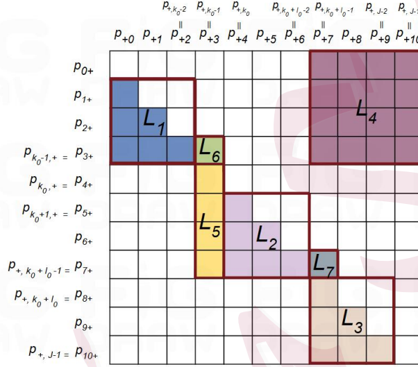
Figure 1: Matrix visualization for J = 11 , k_0 = 4 , l_0 = 4 , and M = 1 . The matrix is partitioned into seven blocks determined by (k_0, l_0) ; unshaded entries are zero. Row markers on the left indicate p_{k+}^{[m]} and column markers on the top indicate p_{+l}^{[m]} for L_{[m]}^* .
