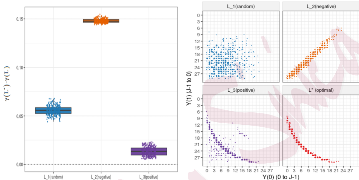
(a) Box plot of \gamma(L^*) - \gamma(L) , matrix construction from left to right: L_1 (random), L_2 (negative), L_3 (positive)
