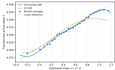
Figure 4: Fitted links for the DC and full-sample estimators.
