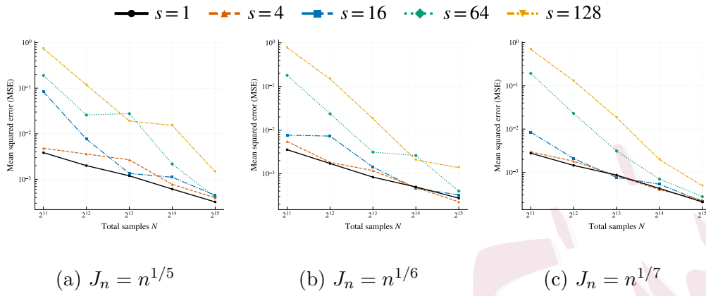
Figure 1: Average MSE of the aggregated estimator \bar{f} under different choices of s and N , with curves to different numbers of machines s .
