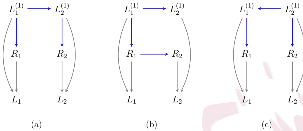
Figure 1: Three possible structures satisfy Assumption 1.
