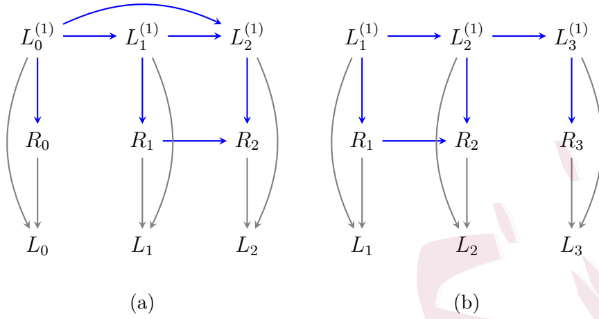
Figure 3: Some identifiable m-DAGs with baseline and follow-up measurements.
