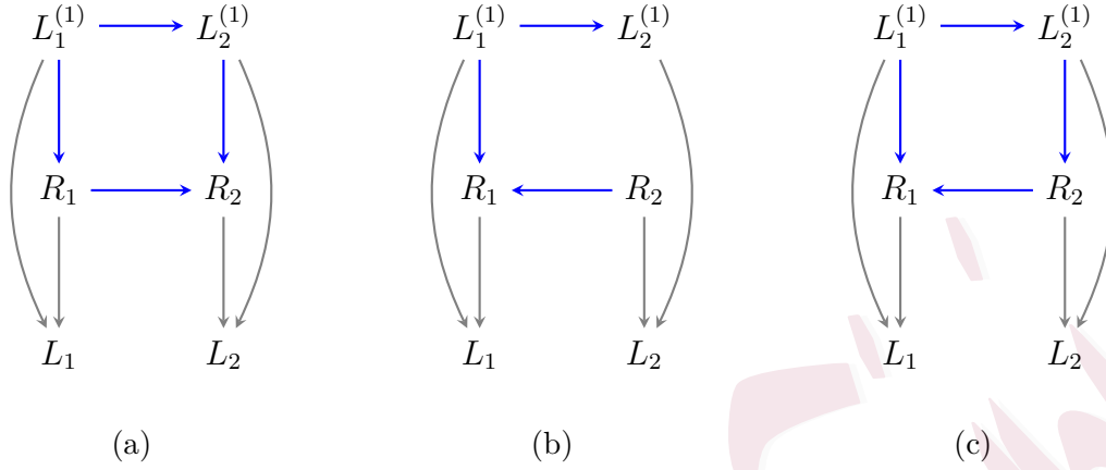
Figure 2: Three possible structures do not satisfy Assumption 1.
