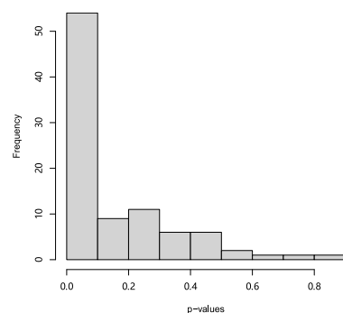
Figure 2: Histogram of the p-values of the Box-Pierce test for all residual sequences.
