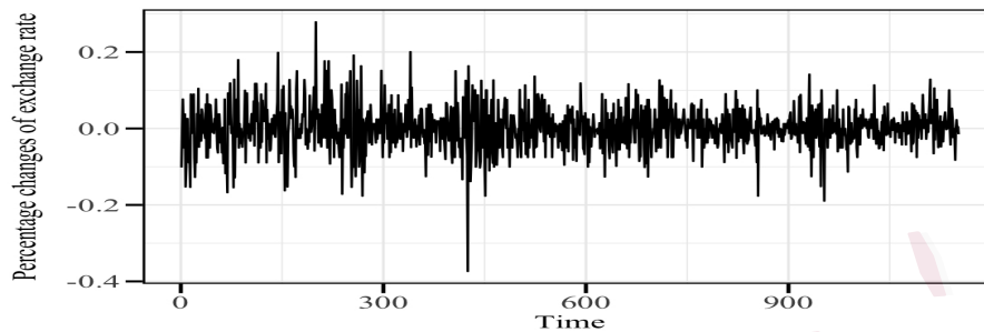
Figure 2: Time series plot of the percentage changes of the exchange rate between the mark and dollar in 10-min intervals: time series length, 1152.
