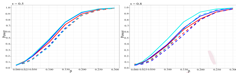
Figure 1: Simulated power of the likelihood ratio test with/without inequality constraints (solid/dashed blue), the rank-based test with/without inequality constraints (solid/dashed cyan), the Wald test with/without inequality constraints (solid/dashed red) under Setting (iii).
