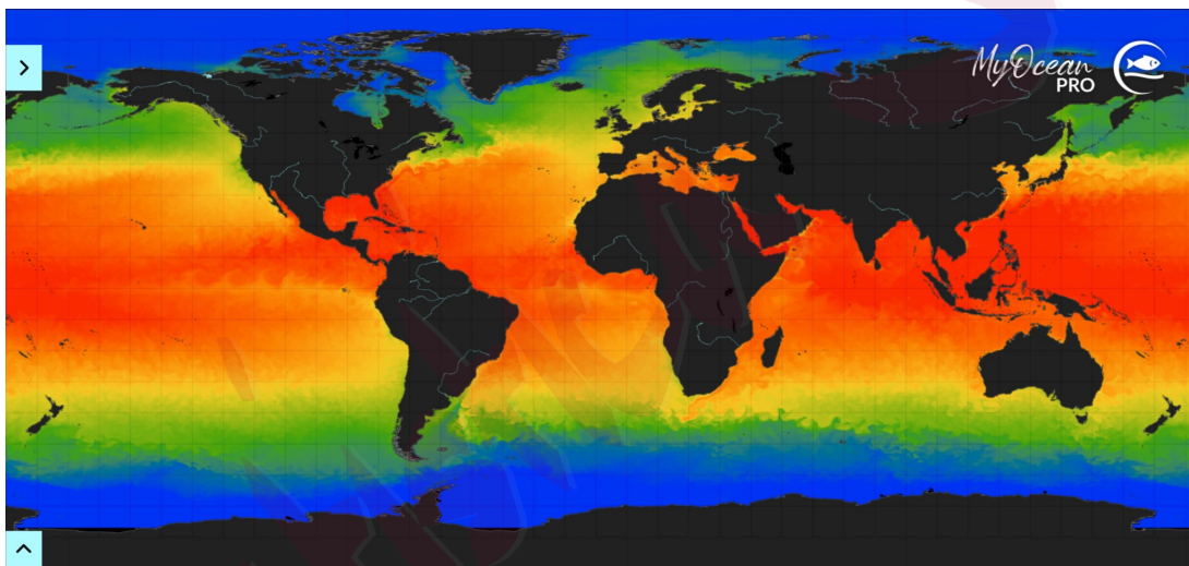
Figure 1: Heat map of global ocean temperature on 2024/7/1 at 20:00.
