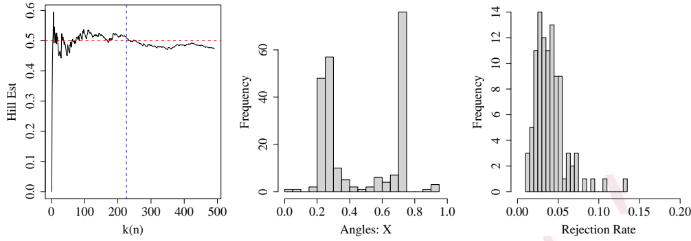
Figure 3: Left: Hill plot of |x| + |y| ; the red line denotes 1/\alpha = 0.5 and the blue line denotes k(n) = 226 . Middle: Histogram of \Theta_1 with n = 2,500 and k(n) = 226 . Right: Histogram of rejection rates of H_0^{(1)} : S([\hat{a}, \hat{b}]) = 1 by \hat{D}_m among 100 simulated trials.
