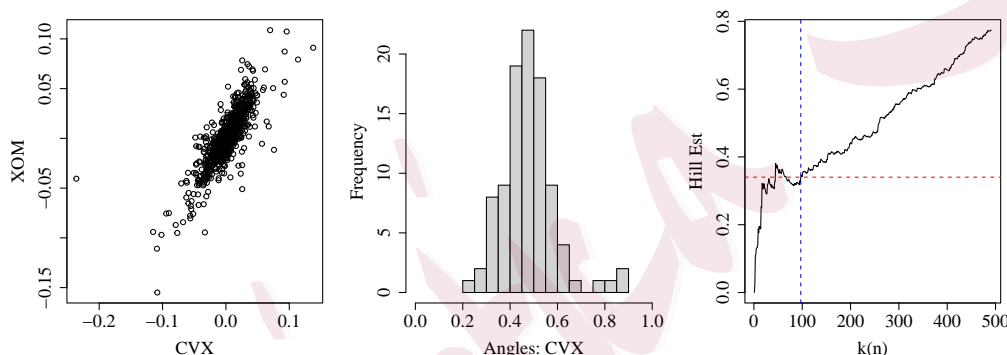
Figure 6: CVX vs XOM. Left: Scatter plot of CVX and XOM returns. Middle: Histogram of angles (absolute returns of CVX) with k(n) = 97 . Right: Hill plot of |x| + |y| .
