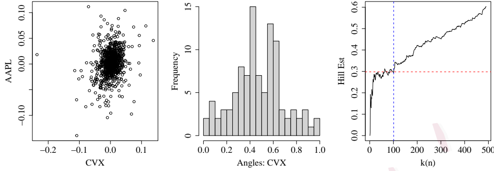
Figure 7: CVX vs AAPL. Left: Scatter plot of CVX and AAPL returns. Middle: Histogram of angles (absolute returns of CVX) with k(n) = 101 . Right: Hill plot of |x| + |y| .
