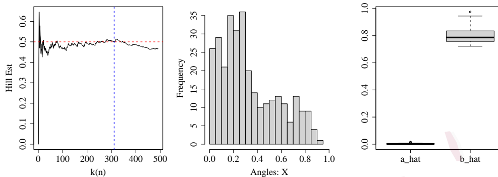
Figure 4: Left: Hill plot of |x| + |y| , and the red line denotes 1/\alpha = 0.5 . Middle: Histogram of \Theta_1 with n = 2,500 and k(n) = 311 . Right: Boxplot of \hat{a} and \hat{b} among 100 simulated trials.
