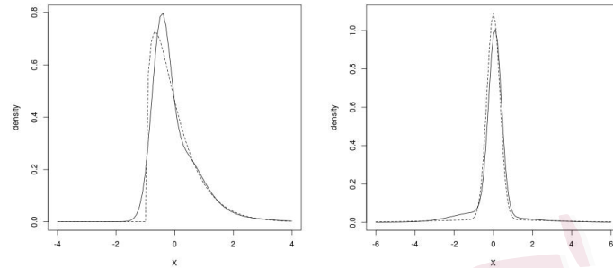
Figure 1: Plot for the nonparametric fit for density of G . The left hand panel shows a typical fit for shifted Gamma distribution for skewed G , the right hand panel is a typical fit in example 1 with a = 10 . The solid line is the fitted and the dashed line is the true target density.
