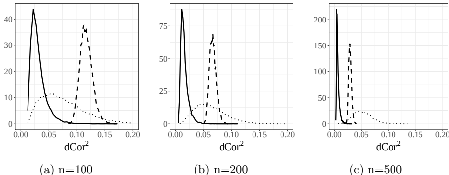
Figure 1. Distribution of dCor^2_n(X_1, Y) (solid line, for a 1-dim inactive variable), dCor^2_n(X_2, Y) (dotted line, for a 20-dim inactive variable), and dCor^2_n(X_3, Y) (dash line, for 1-dim active variable).
