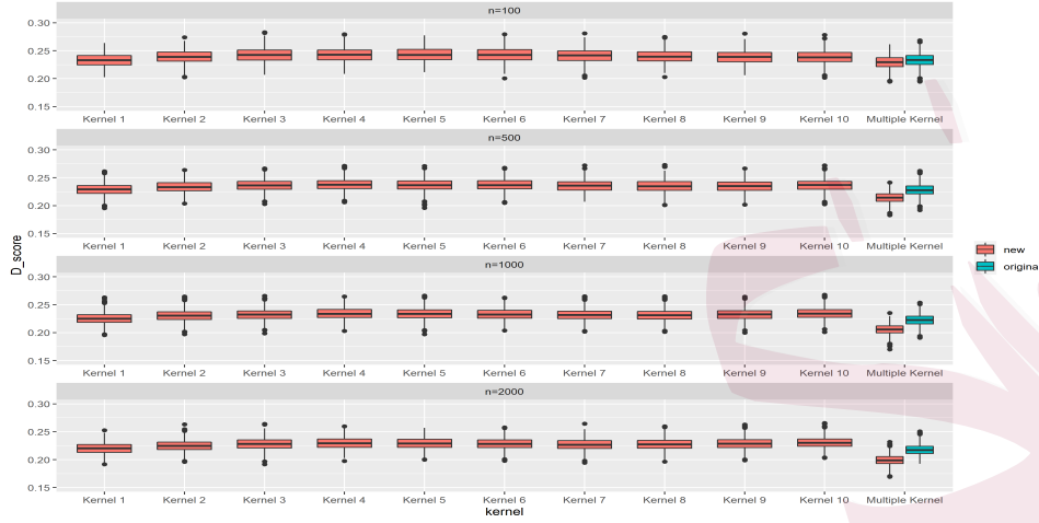
Figure 4: Boxplots of D(\Omega, \hat{\Omega}) for the proposed method using the 10 kernels (new) in (4.24), or each of those 10 kernels (Kernel 1, \dots , Kernel 10), and the method of Bachoc et al. (2020) using the 10 kernels (original) in a simulation with 1000 replications for the non-Gaussian random fields. The number of observations n is 100, 500, 1000 or 2000 (from top to bottom), and the dimension of random fields is p = 50 .
