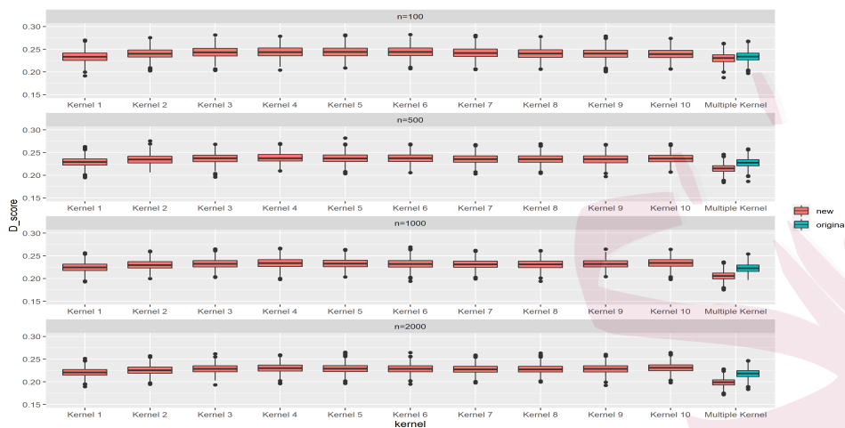
Figure 3: Boxplots of D(\Omega, \hat{\Omega}) for the proposed method using the 10 kernels (new) in (4.24), or each of those 10 kernels (Kernel 1, \dots , Kernel 10), and the method of Bachoc et al. (2020) using the 10 kernels (original) in a simulation with 1000 replications for the Gaussian random fields. The number of observations n is 100, 500, 1000 or 2000 (from top to bottom), and the dimension of random fields is p = 50 .
