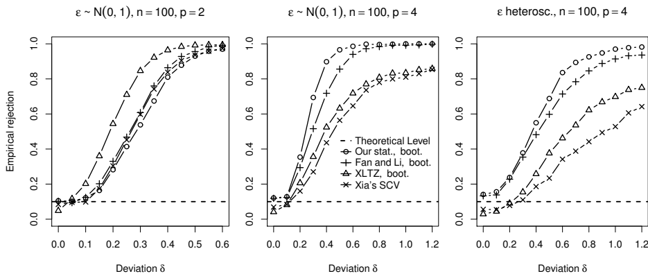
Figure 2: Power curves for model (5.1), n = 100
