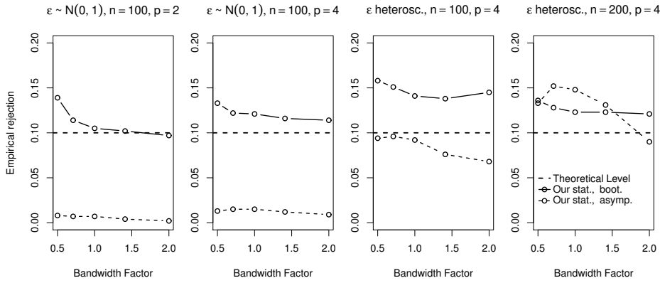
Figure 1: Empirical rejections under H_0 as a function of the bandwidth. \varepsilon
