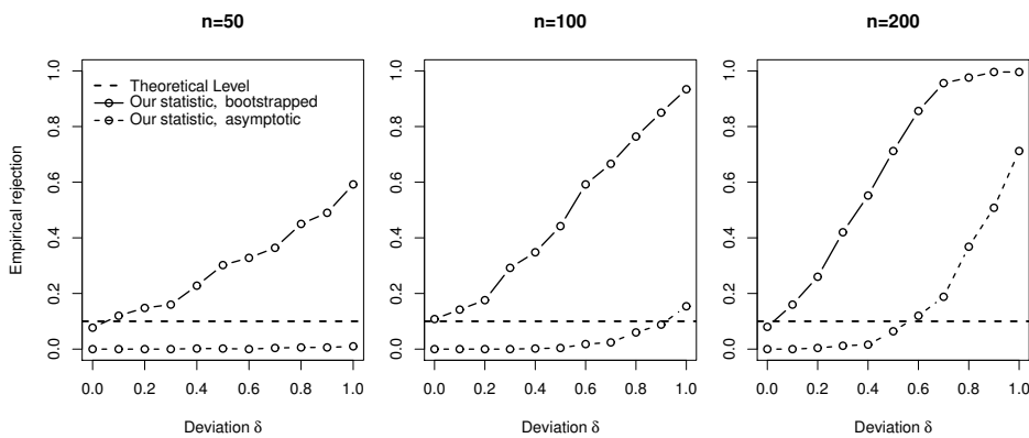
Figure 4: Power curves for model (5.3).
