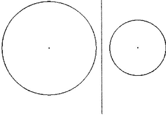
等幂軸
